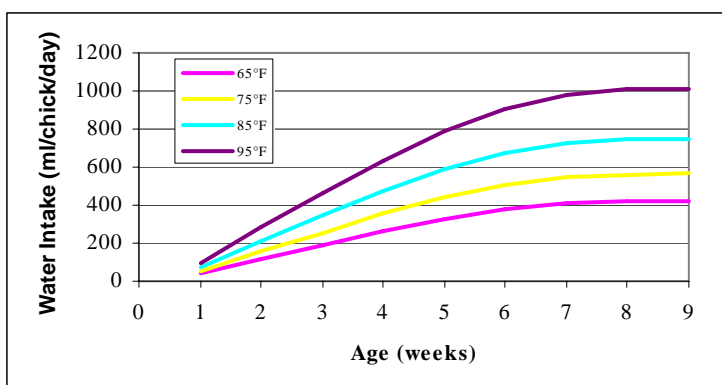
Figure 2: Effect of Environmental Temperature on Water Intake. (Based on daily feed consumption defined in the Ross Broiler Performance Objectives , June 2007 and the assumption that water intake increases by 3.33% per °F increase in temperature [6% per °C], Singleton, 2004).
